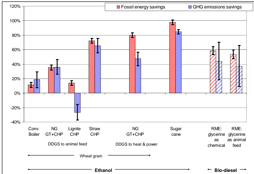
Fig. A1.1: JEC-WTW estimates of direct GHG saving and fossil-energy savings from replacing fossil fuel with different biofuels. Indirect effects are not included. Results depend on plant configuration and use of by-products. Brazilian sugar cane is better because bagasse waste heats the process. Error bars represent technical uncertainties, mainly from estimation of nitrous oxide emissions.
